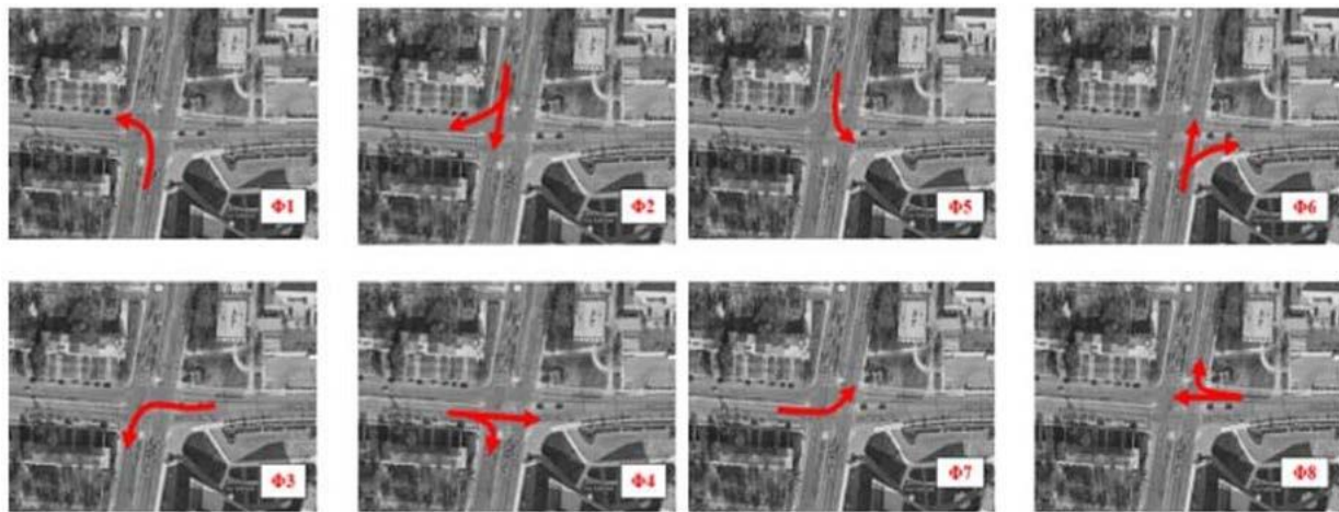
Figure 18 Different Phases of The Traffic Signal
